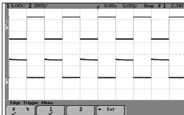
Fig3 : up : modulation signal; down : resulting intensity signal. Response at 50Hz. No thermal effect thanks to unloaded capacitive electrodes
