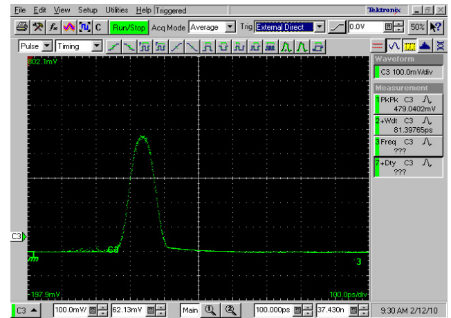
Generated 80 ps Optical Pulse
