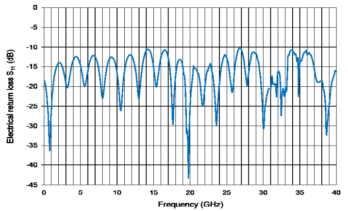
MXAN1300-LN-20 Typical S_{11} Curve
