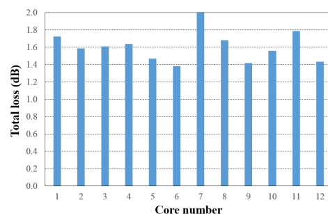
Fig. 6. End-to-end loss measured at 1.31 \mu\text{m} for each core (combiner + 12c-EYDF + combiner)
