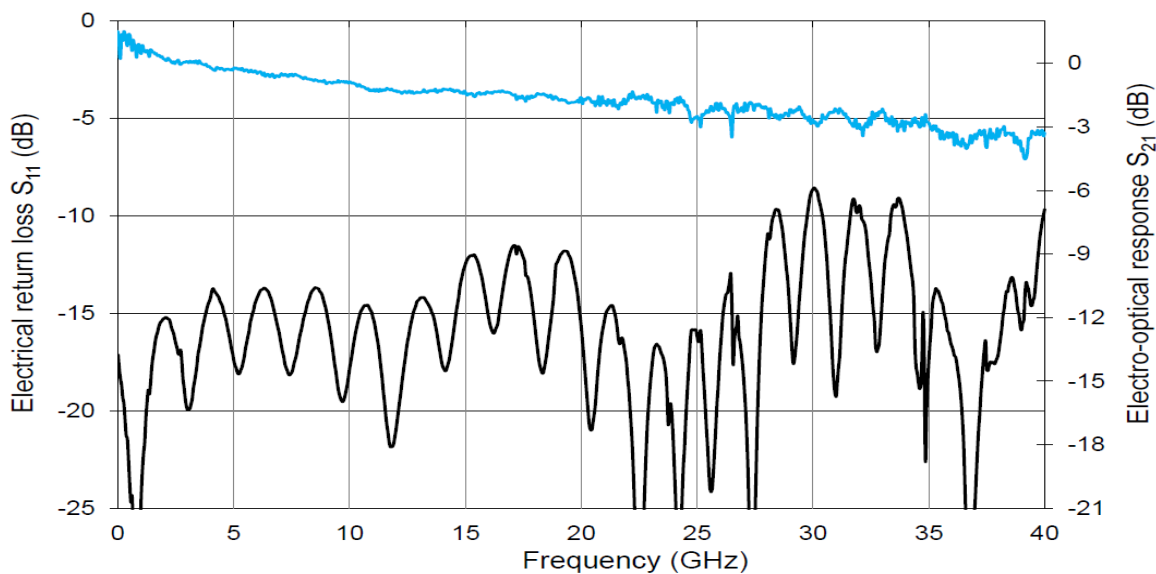
Typical Curve S_{21} & S_{11} from RF 2 Electrode
