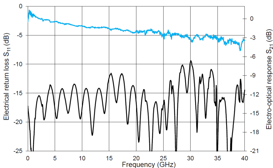
Typical Curve S_{21} & S_{11} from RF 1 Electrode
