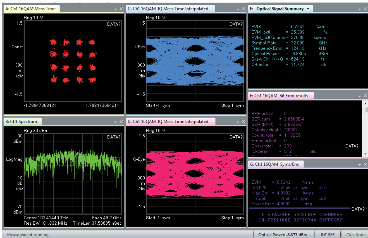
16QAM- 32 Gbaud/s
